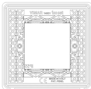
Backside view
