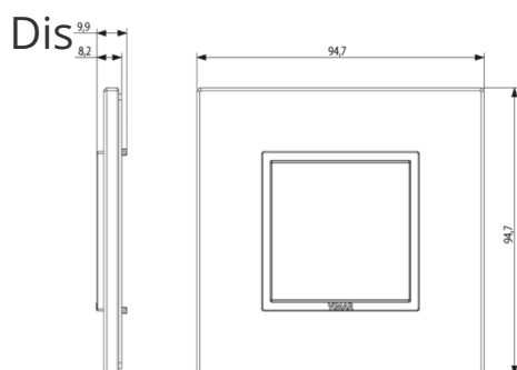
21602 - Frame 2M +claws 71mm
