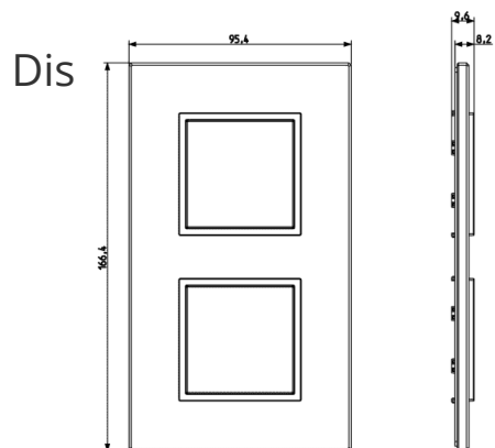
21603 - Frame 2M without screws 71mm
