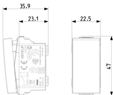
09013 - 1P 16AX reversing switch white
