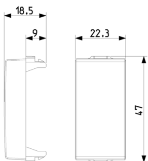
09044 - Cable outlet with cord grip white
