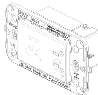
3D View
