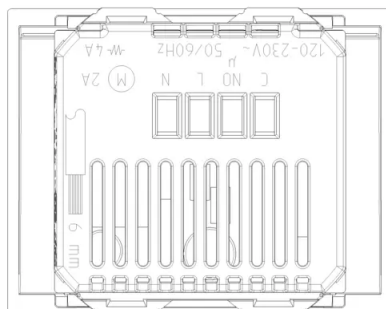
Backside view
