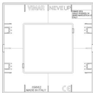
Backside view
