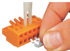
Operating tool for comb-style jumper bars (231-902)
