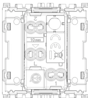
Backside view
