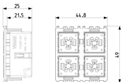
Space view
