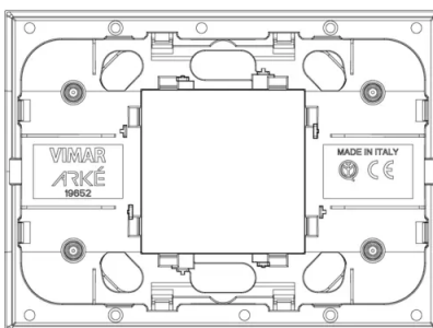
Backside view
