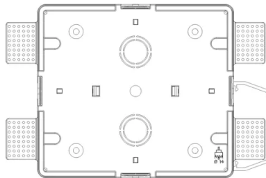
Backside view
