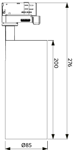
LEDSpot3C-C-P 25W
