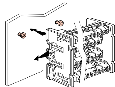
Plate mounting
