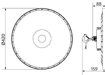
Dimensional_Drawing_HB_E3_180_220W.png
