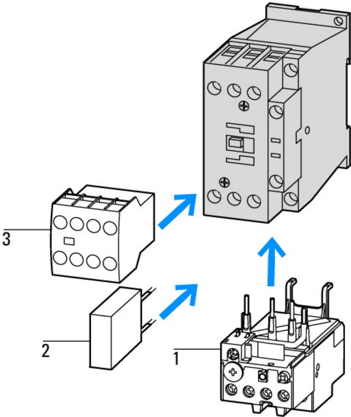
1: Overload relay 2: Suppressor 3: Auxiliary contact modules
