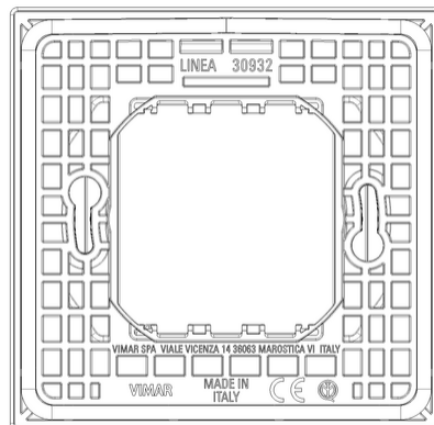
Backside view
