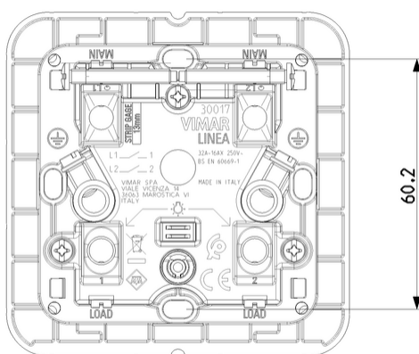
Backside view
