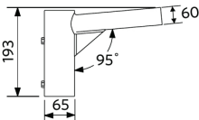
LEDStreetlight Pole-Top-60-Adapter-60
