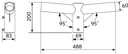
LEDStreetlight Pole-Top-60-Adapter-2x60
