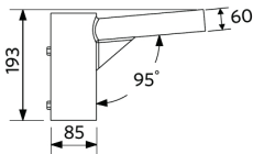
LEDStreetlight Pole-Top-76-Adapter-60
